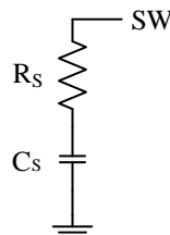
Figure 3 Placement of RC Snubber
