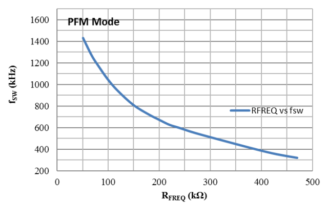
R_{FREQ} vs f_{SW}
