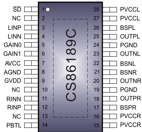
(TSSOP28-PP)PACKAGE (TOPVIEW)
