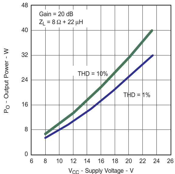
OUTPUTPOWER vs SUPPLYVOLTAGE(BTL)
