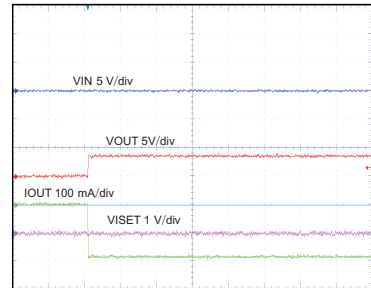
20- \Omega resistor at OUT.No input.VBAT=3.7V Battery PlugIn
