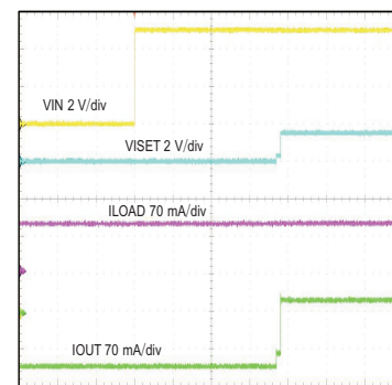
90-mA Load,120-mA ICHG Power Up
