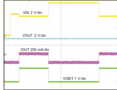
V_{IN} 0V-5V-7V-5V OVPfromNormalPower-UpOperation
