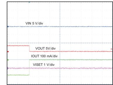
20- \Omega resistor at OUT.No input.VBAT=3.7V Battery Removal
